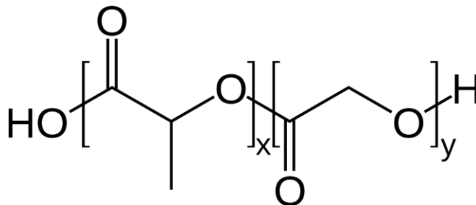
Polymer Synthesis
